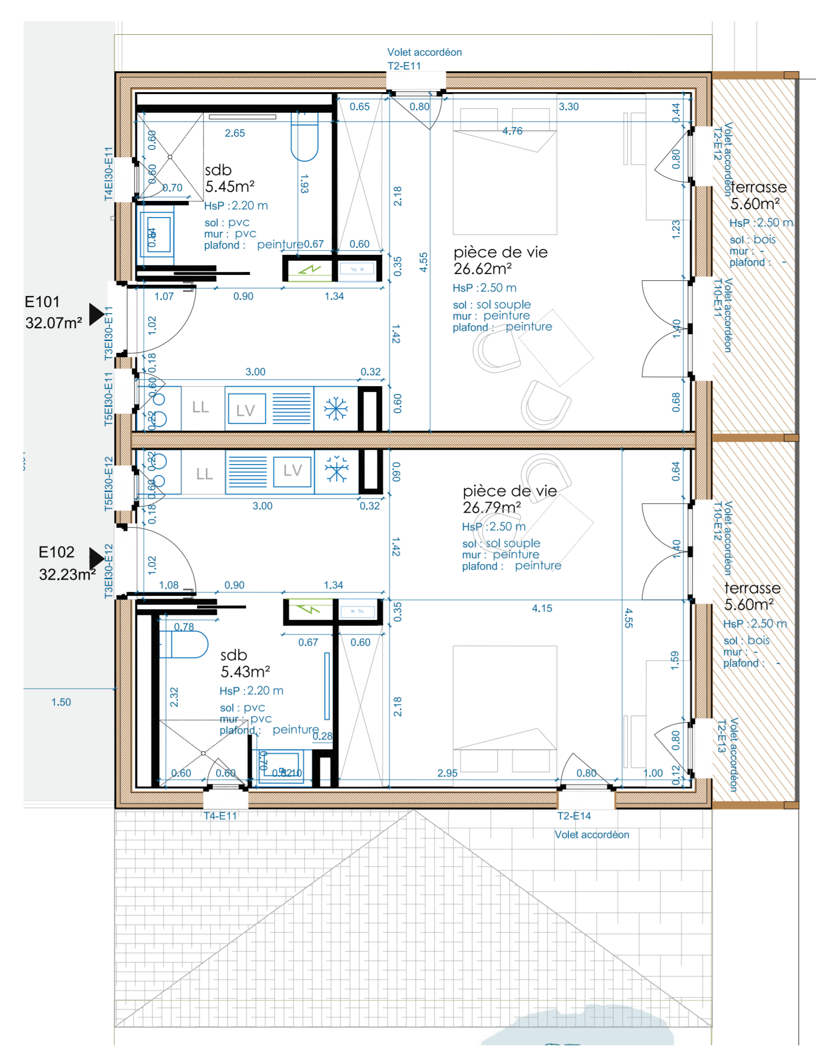
Plan R+1
